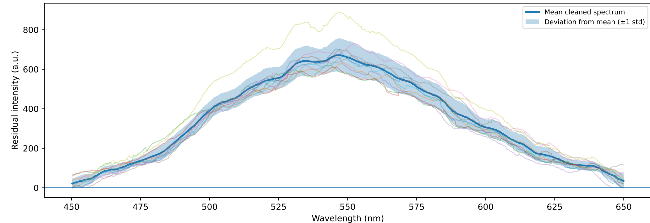
(b) Mean cleaned spectrum after water subtraction with deviation band
