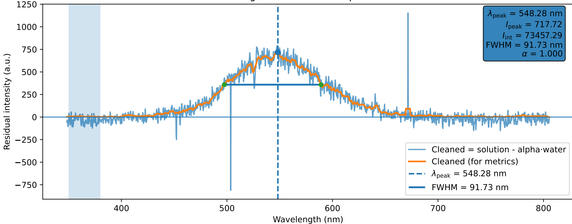
Background-subtracted spectrum
